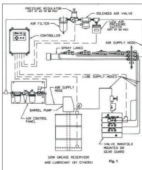
Above: This Bijur Delimon Singline model is a typical automatic spray lubricating system, with pump close to valve panel. Below: A Bijur Delimon system "in a box" for customer demonstrations.
