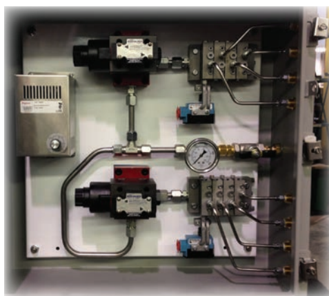
Above: This Bijur Delimon Singline model is a typical automatic spray lubricating system, with pump close to valve panel. Below: A Bijur Delimon system "in a box" for customer demonstrations.
