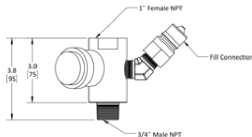
Gearbox Adapter
